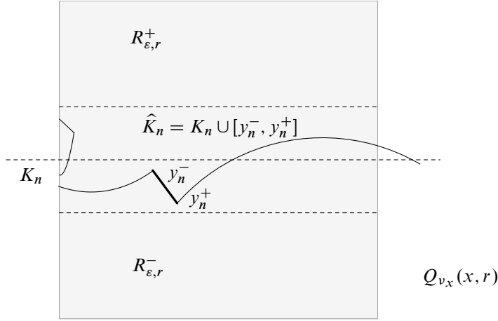
Figure 2. Construction of \widehat{K}_n in Proposition 3.3.
